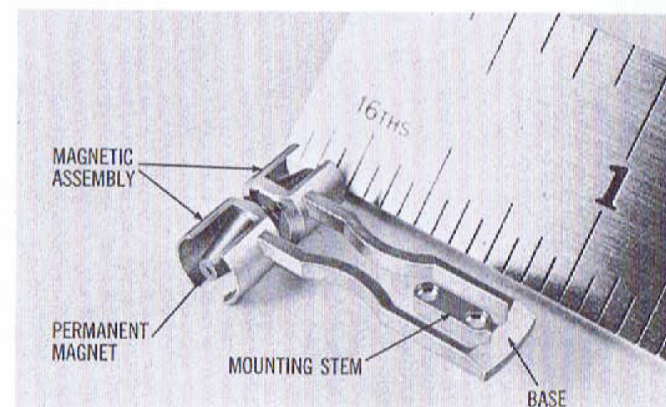
Fig. 9 ACCUTRON Tuning Fork
