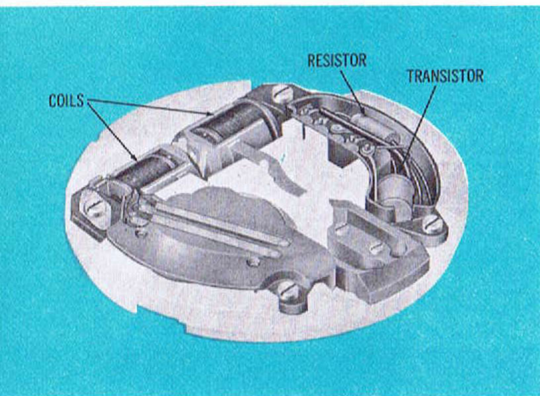
Fig. 10 Tuning Fork and Associated Circuit Elements (Front View)
