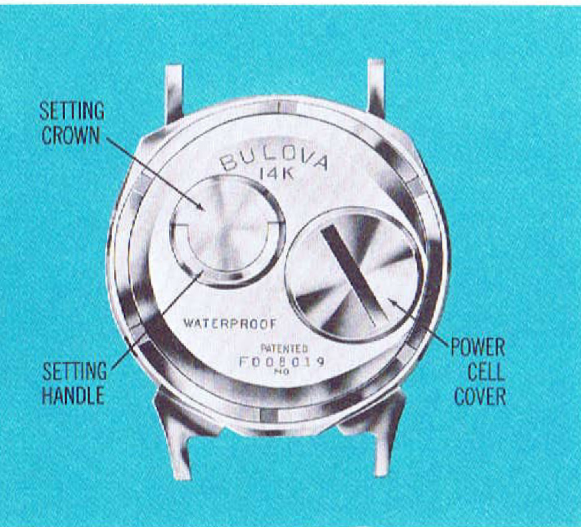
Fig. 1 Rear View of ACCUTRON Case
