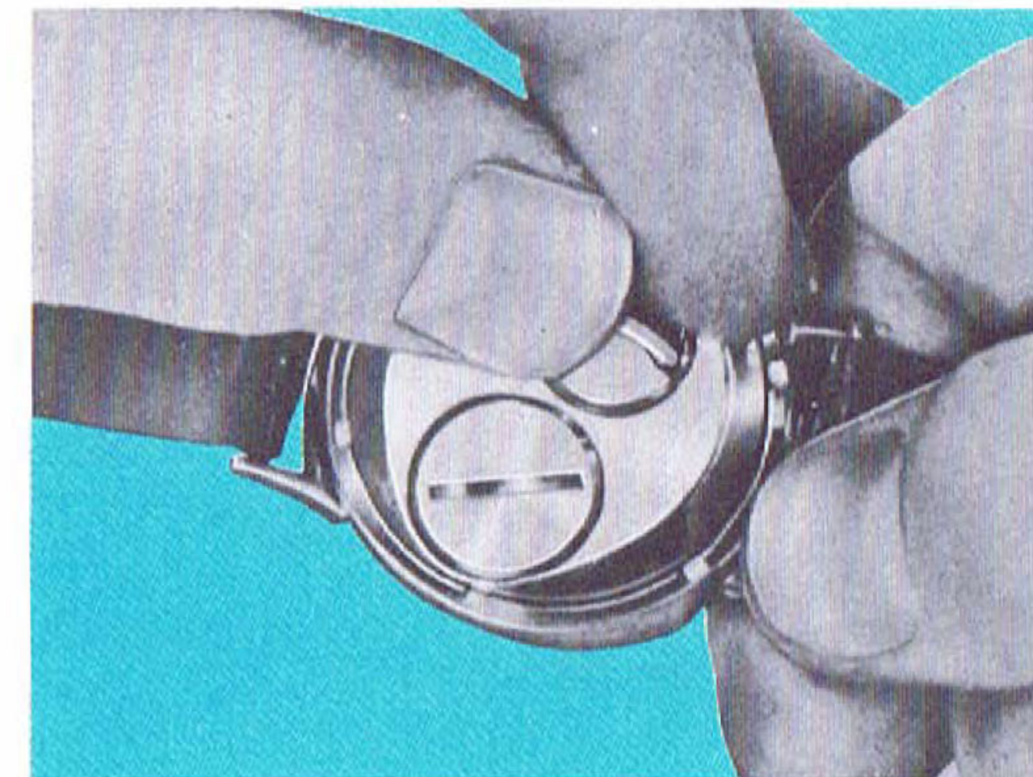
Fig. 3 Setting the Hands
