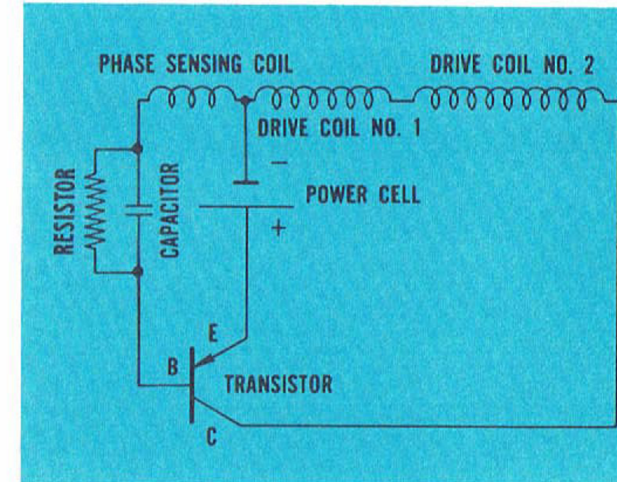
Fig. 15 Schematic Diagram of ACCUTRON Circuit
