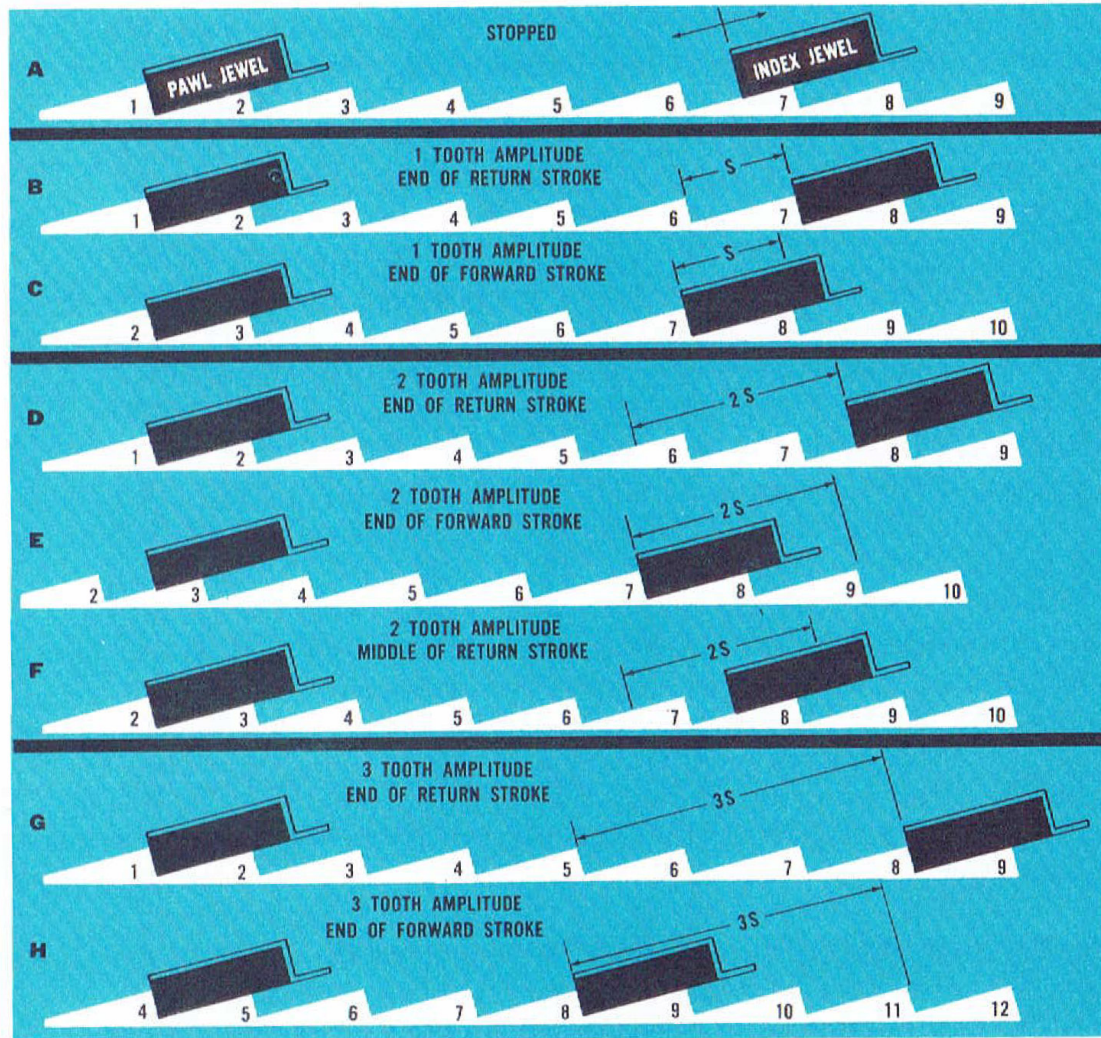
Fig. 13 Diagram of Indexing Mechanism Operation
