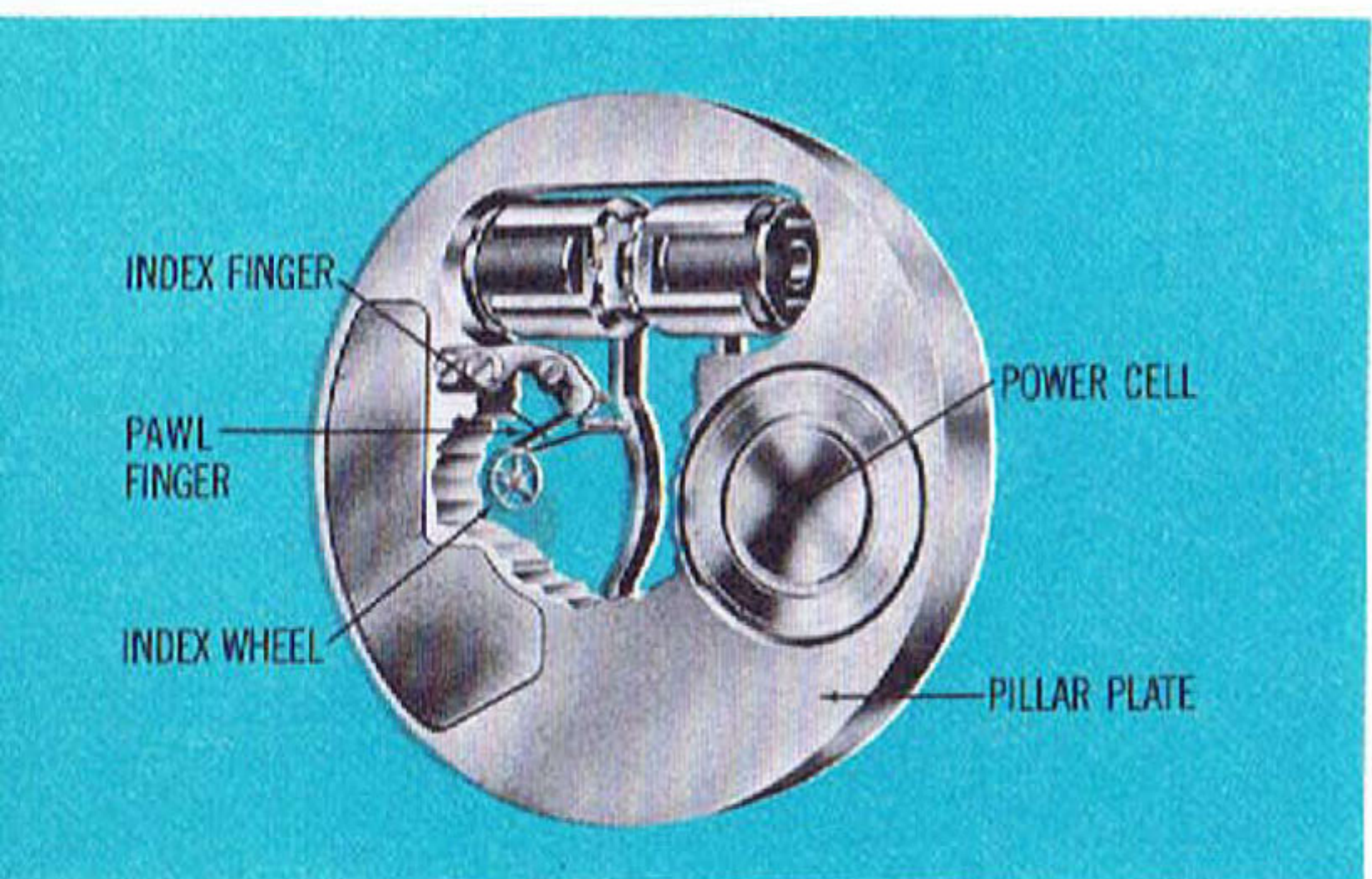
Fig. 11 ACCUTRON Indexing Mechanism (Rear View)
