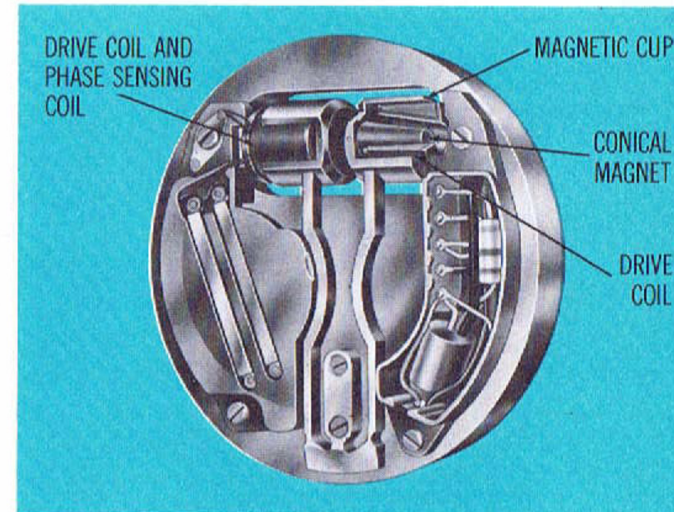
Fig. 14 Cutaway View of ACCUTRON Electro-magnetic Elements
