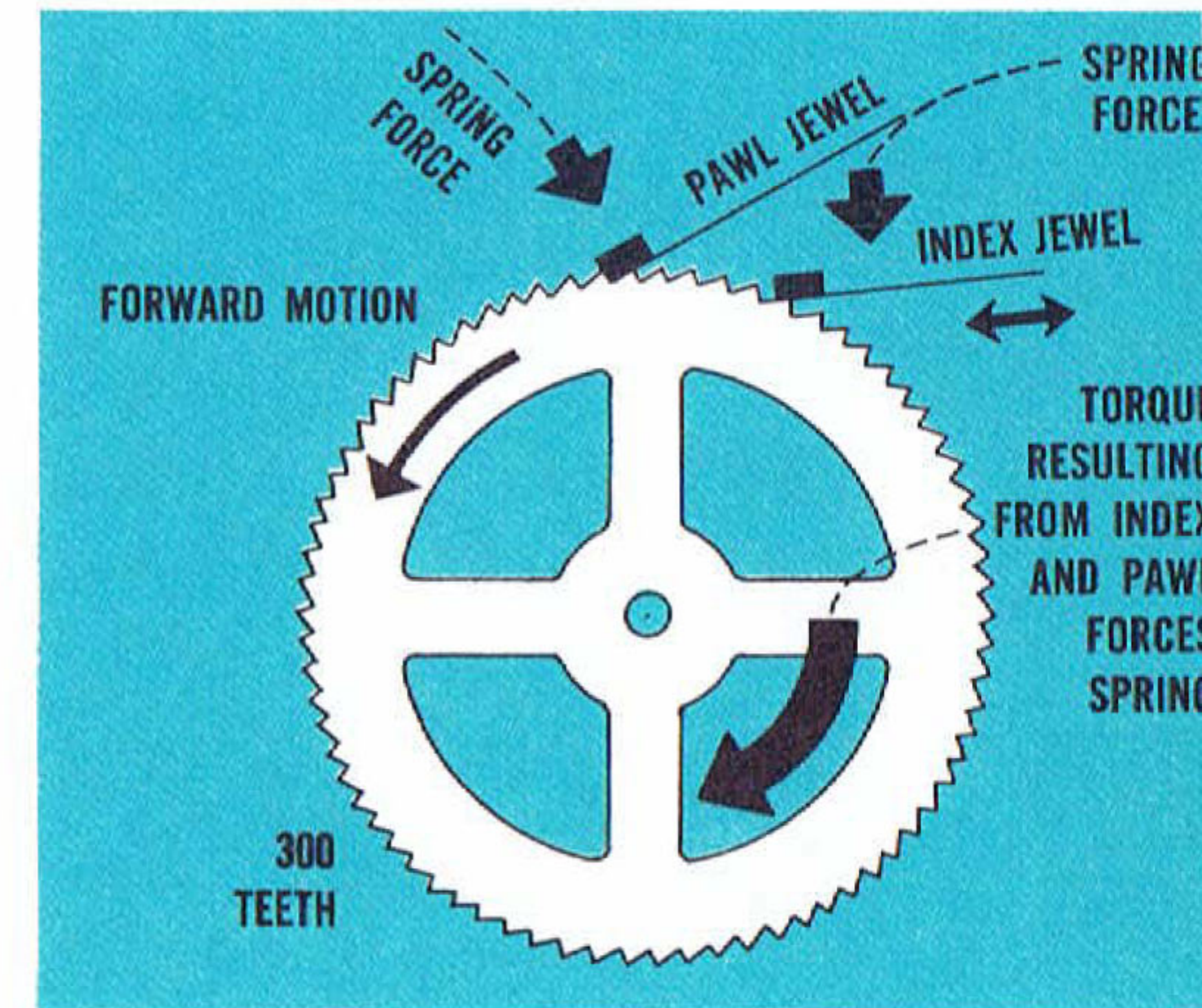
Fig. 12 Diagram of Indexing Mechanism
