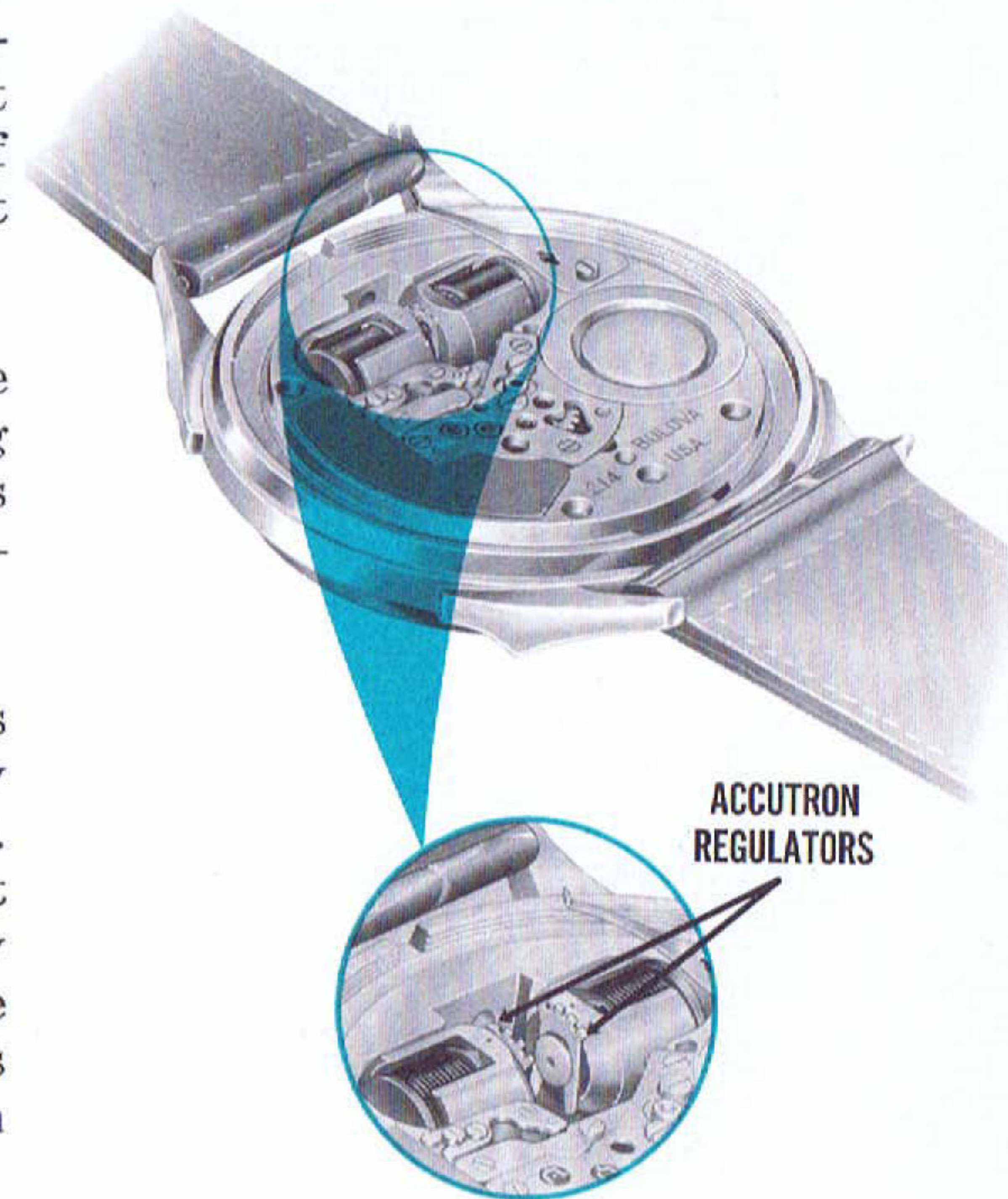
Fig. 6 Rear View of ACCUTRON Movement Showing Regulators
